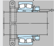
(c) Removal by use of hydraulic nuts
