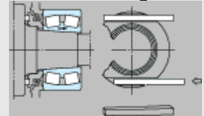
(b) Removal by use of clamps
