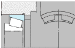
(a) Notches for removal
