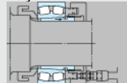
(f) Removal by use of hydraulic nuts
